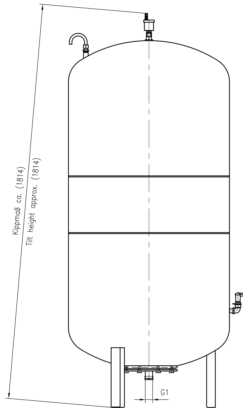
Side view
