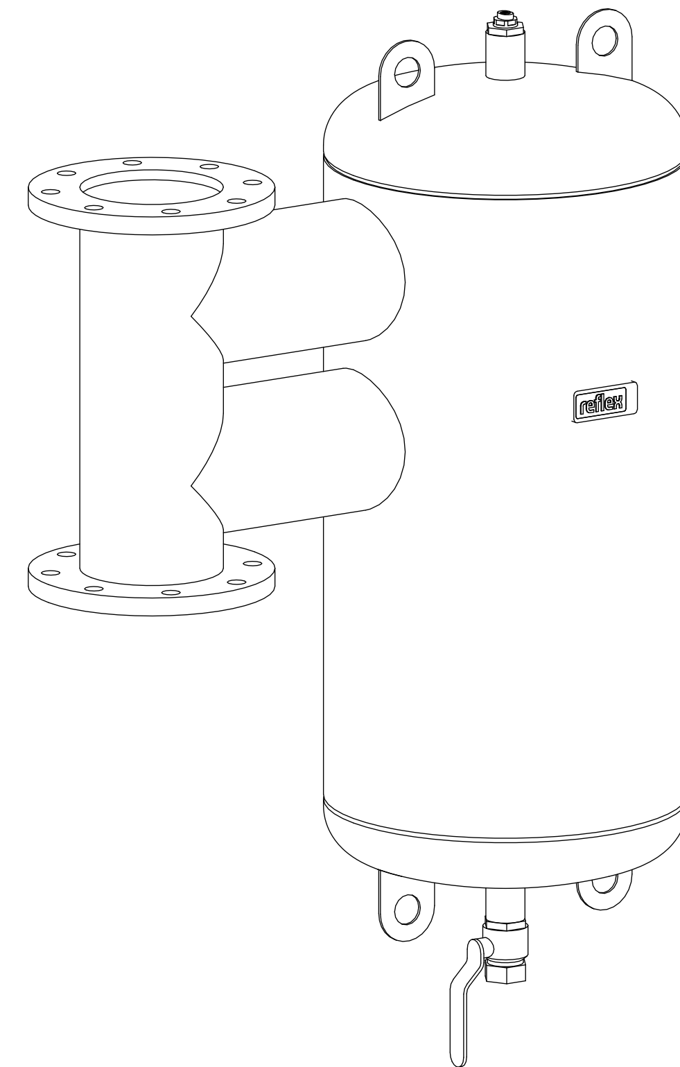
Isometric view
