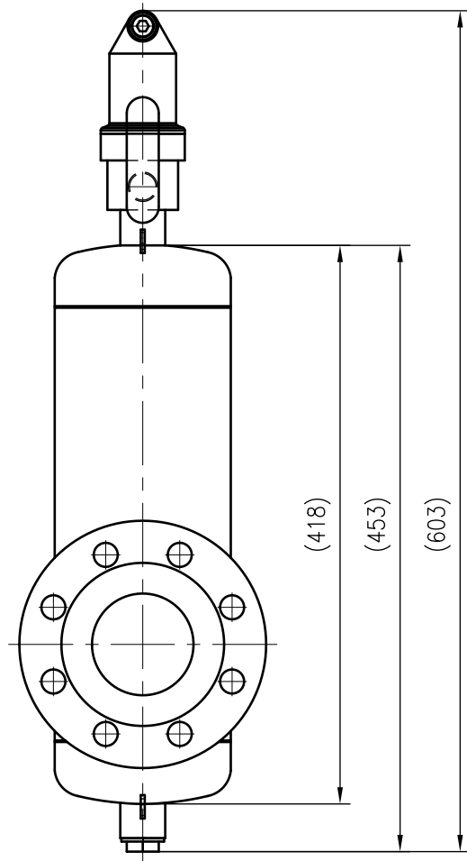
Side view
