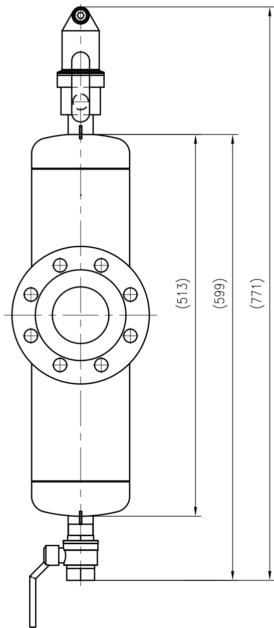
Side view
