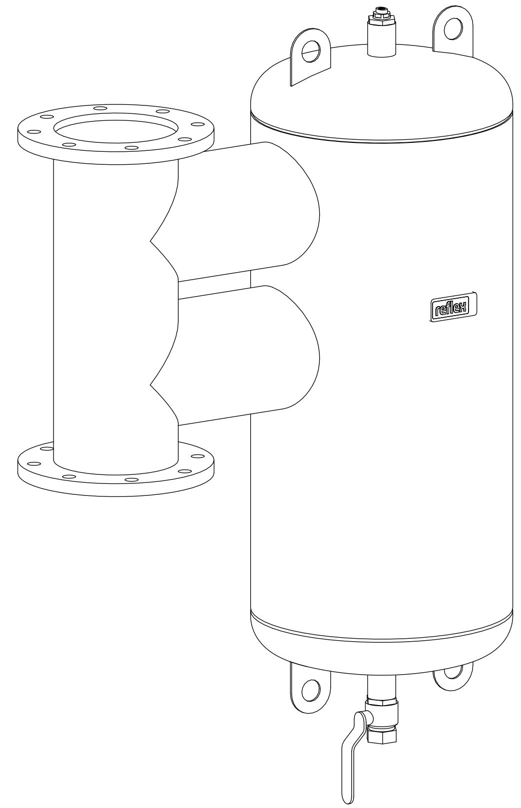
Isometric view
