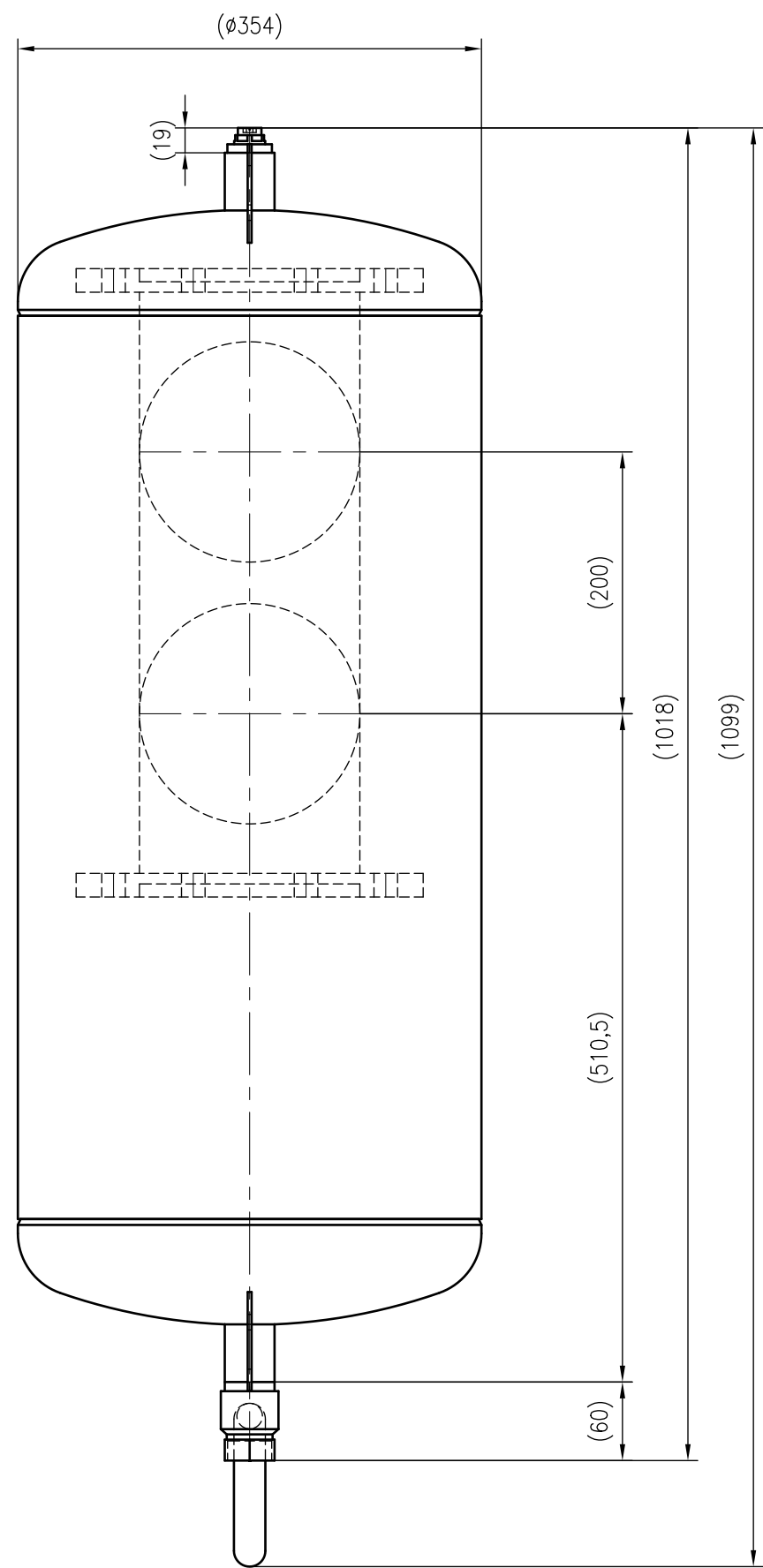
Side view
