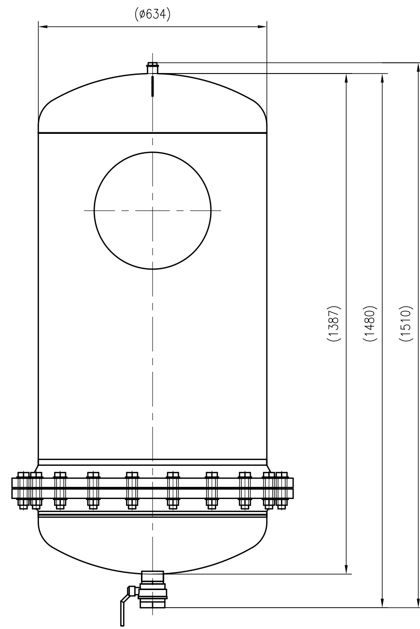
Side view
