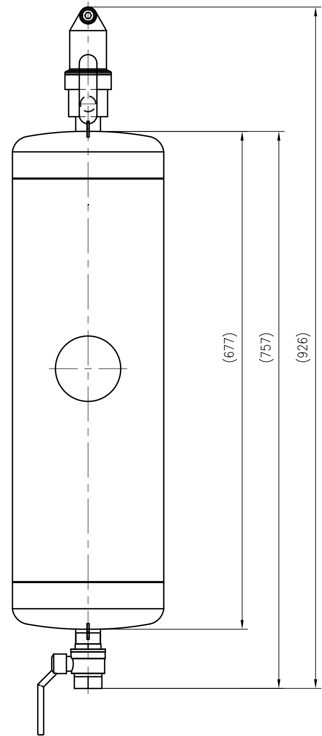
Side view
