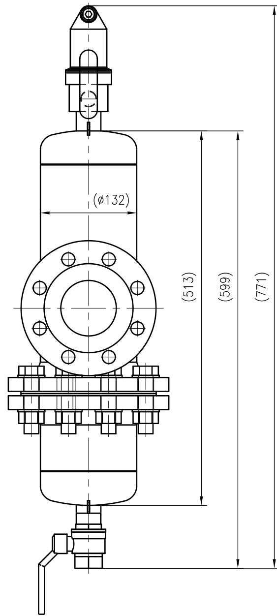
Side view
