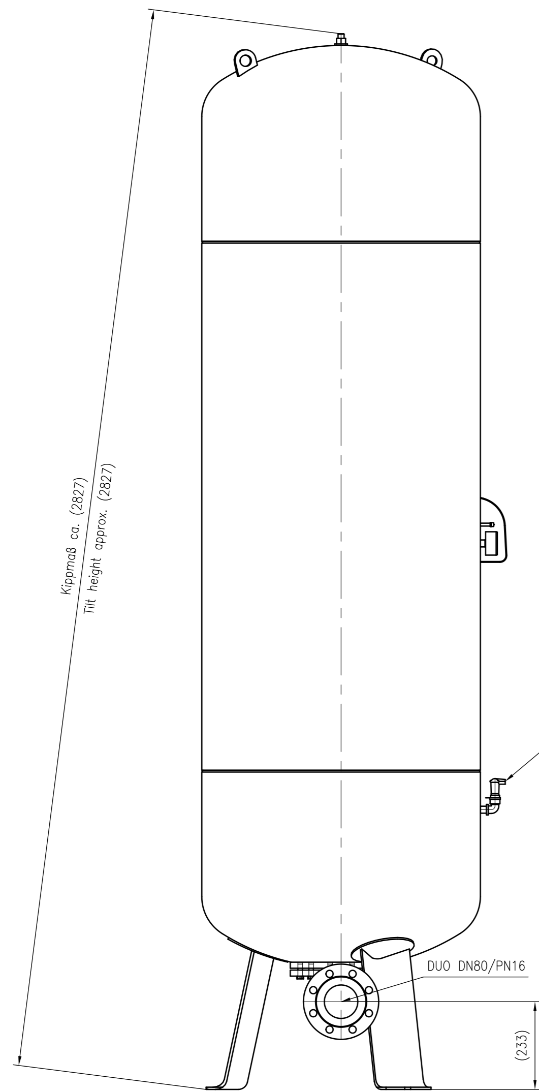
Side view
