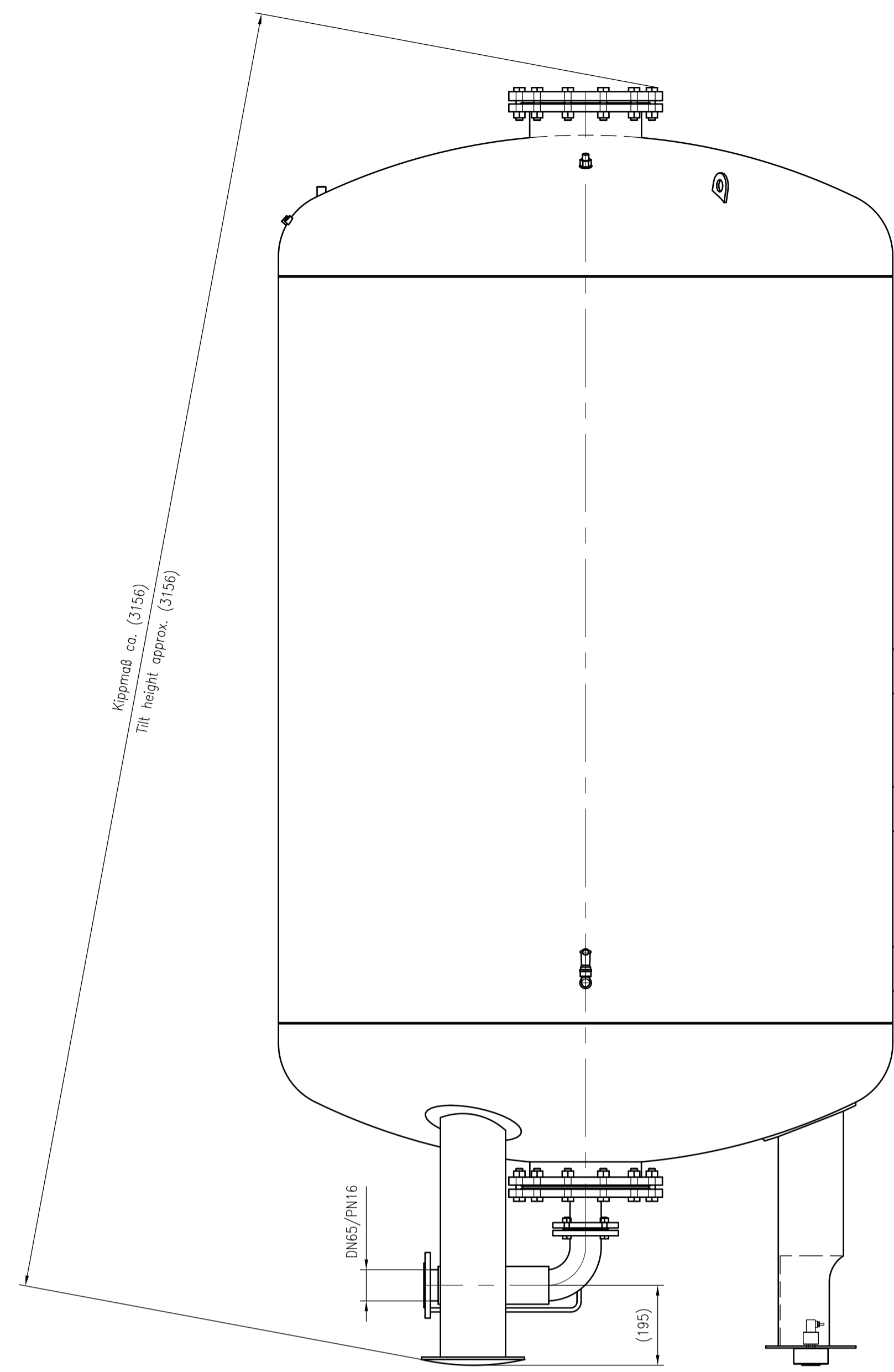
Side view
