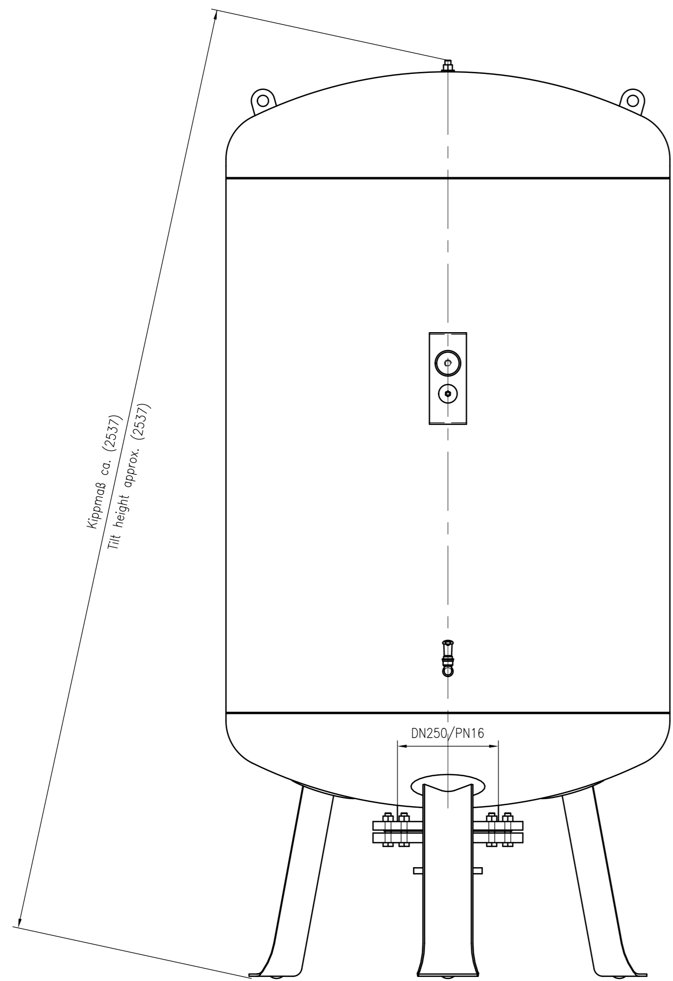
Side view
