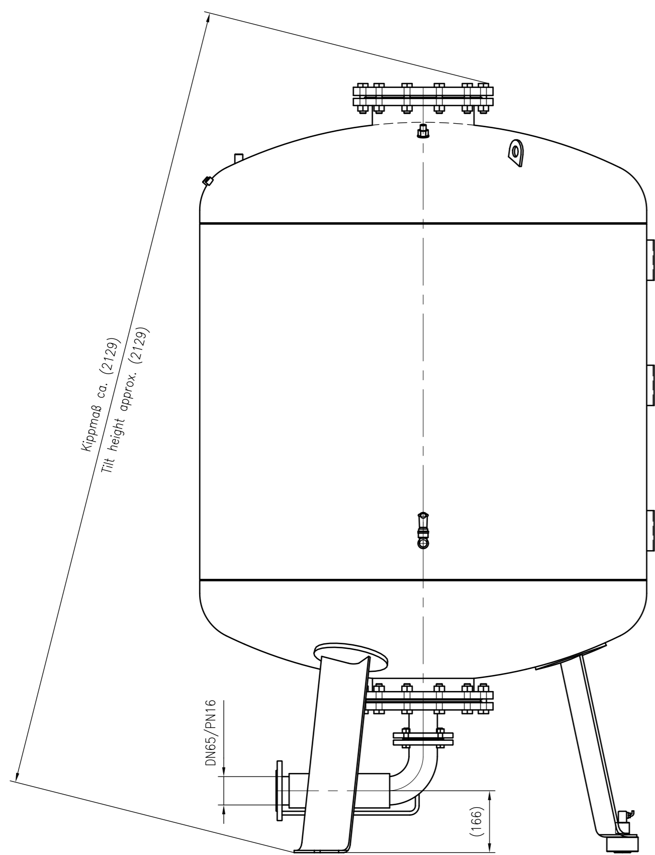
Side view
