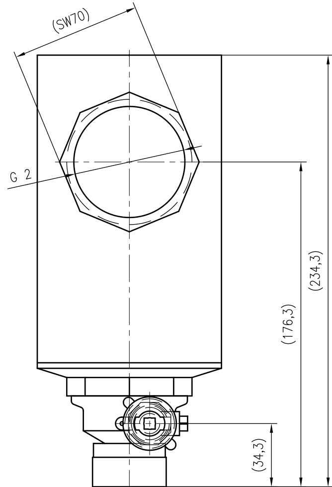
Side view
