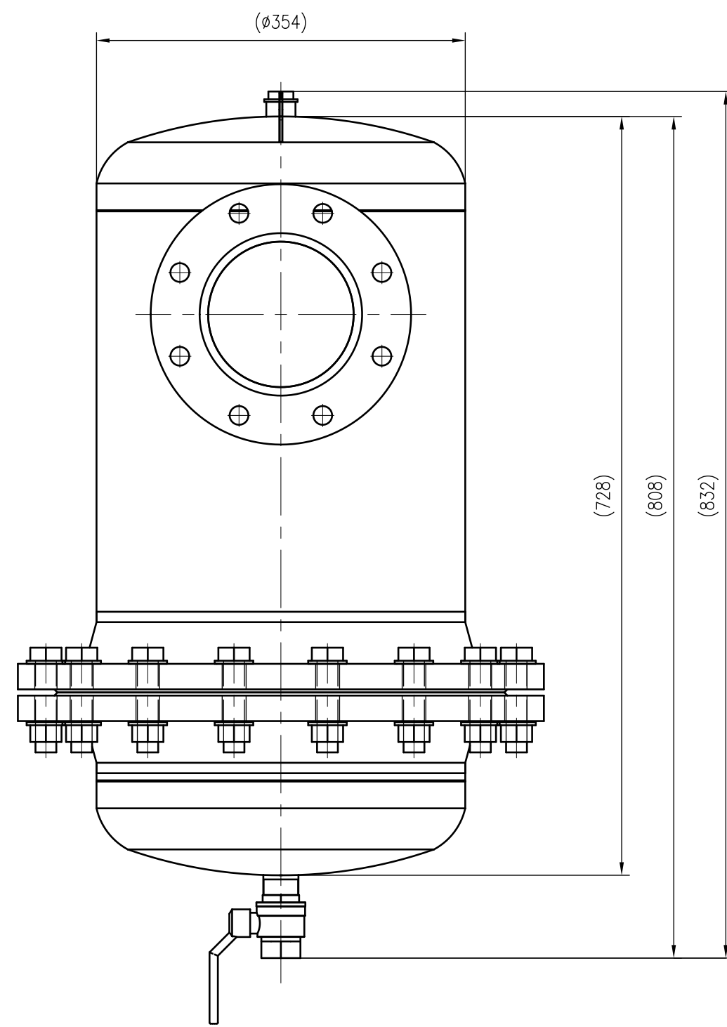
Side view
