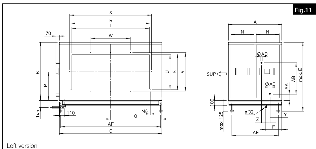
Dimensions change-over-unit DX RH 1500-15000
