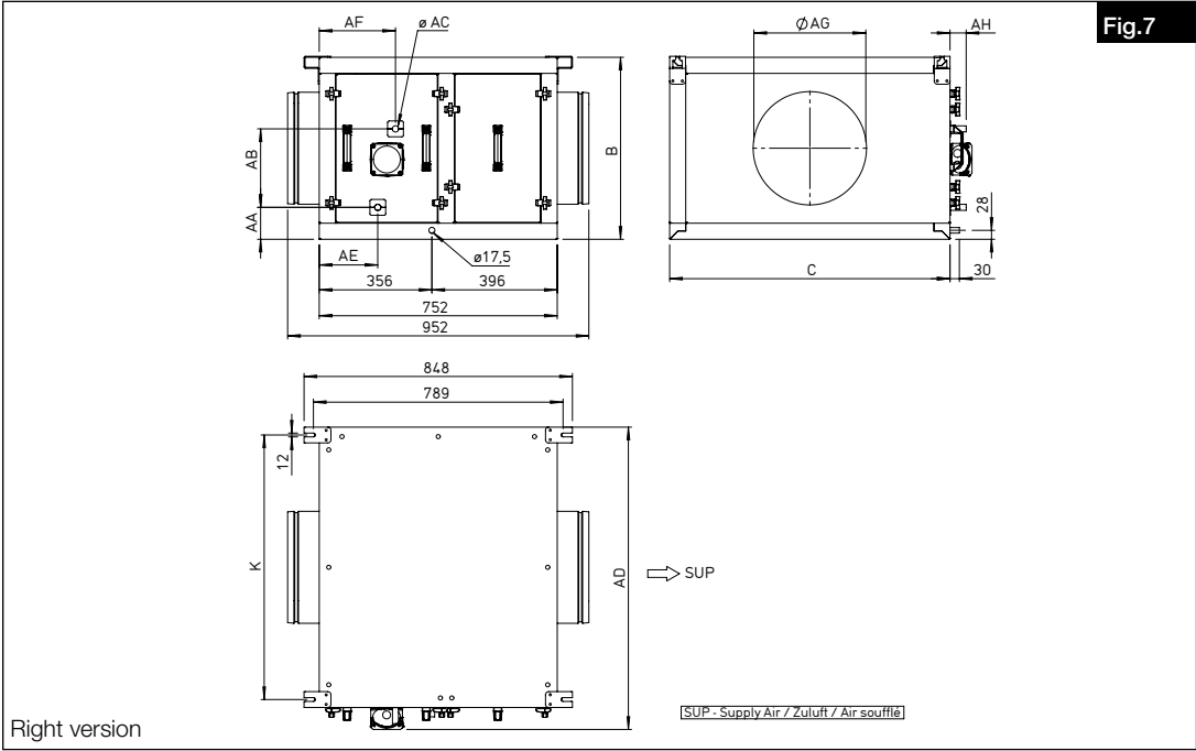
Dimensions change-over-unit DX XVP 850-1800
