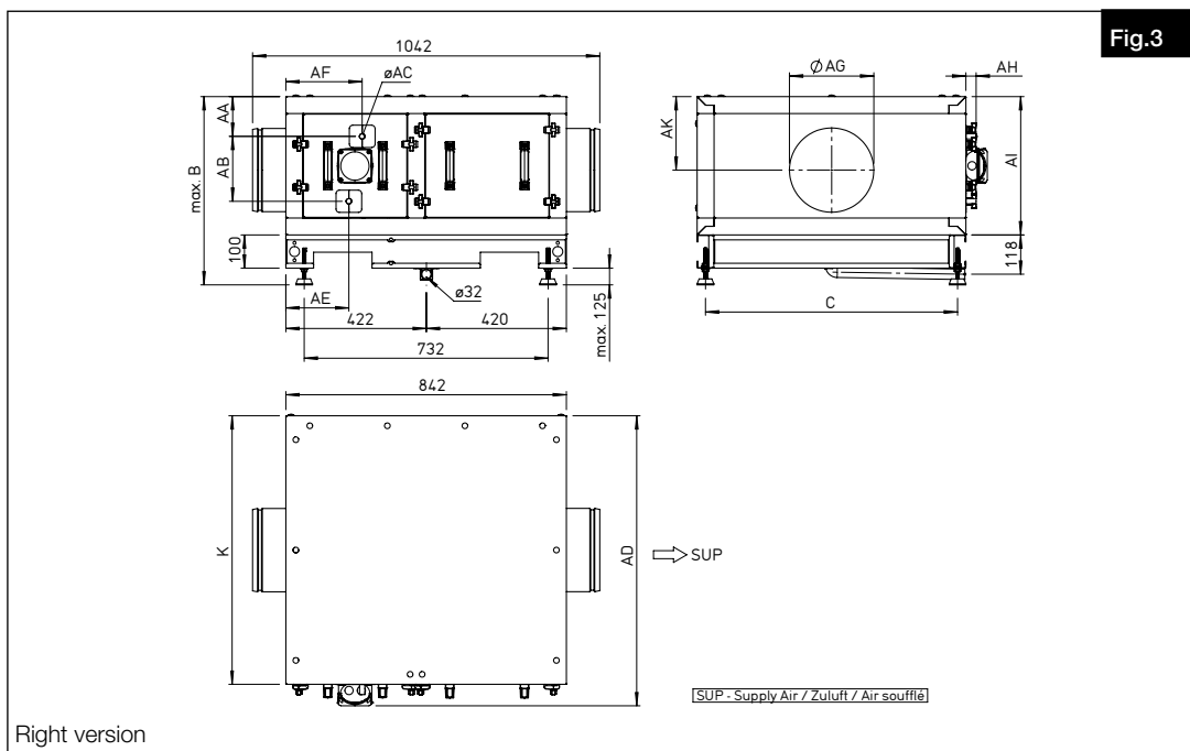
Dimensions change-over-unit DX XHP 750-2500
