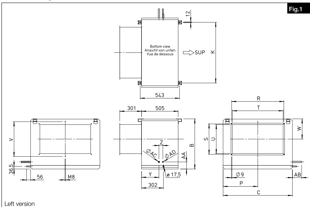
Dimensions change-over-unit DX XC 500-3200
