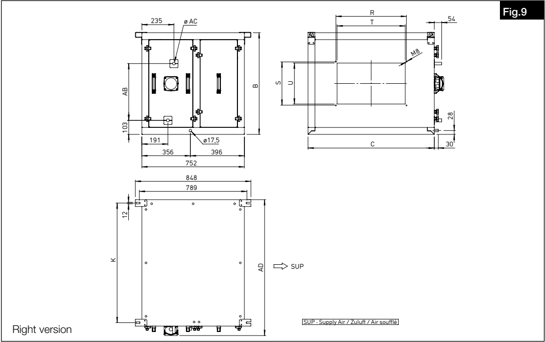
Dimensions change-over-unit DX XVP 2500-3500
