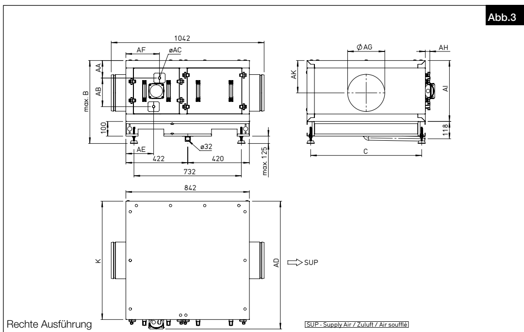
Abmessungen Change-Over-Register DX XHP 750-2500
