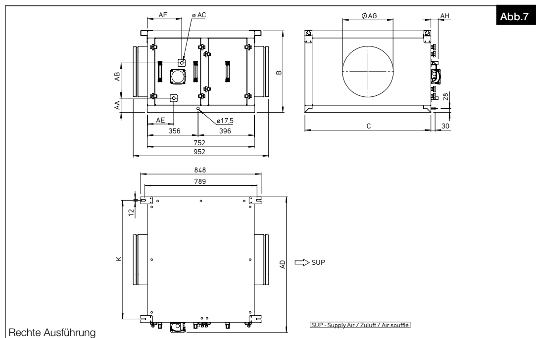
Abmessungen Change-Over-Register DX XVP 850-1800
