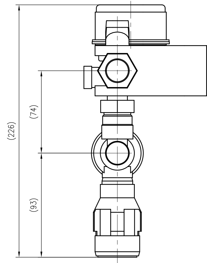
Side view
