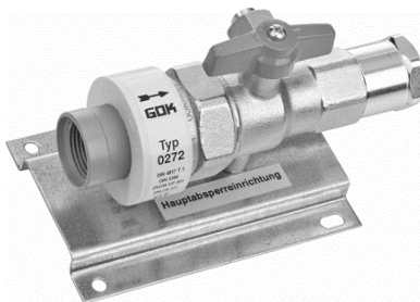
Type 0272 downstream from the house connection
