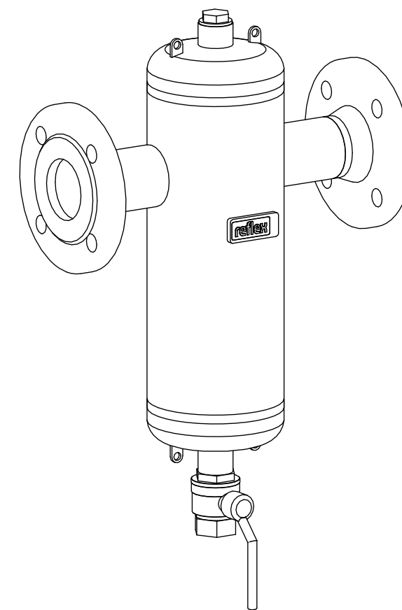
Isometric view
