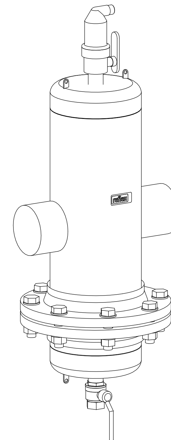
Isometric view
