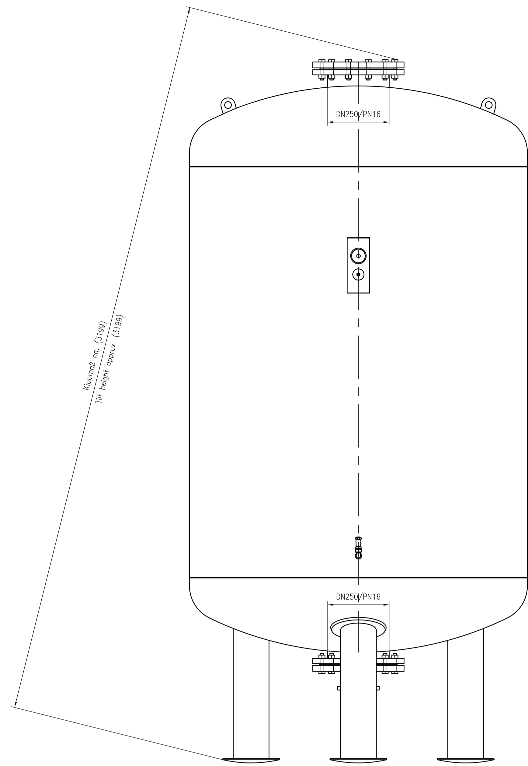
Side view
