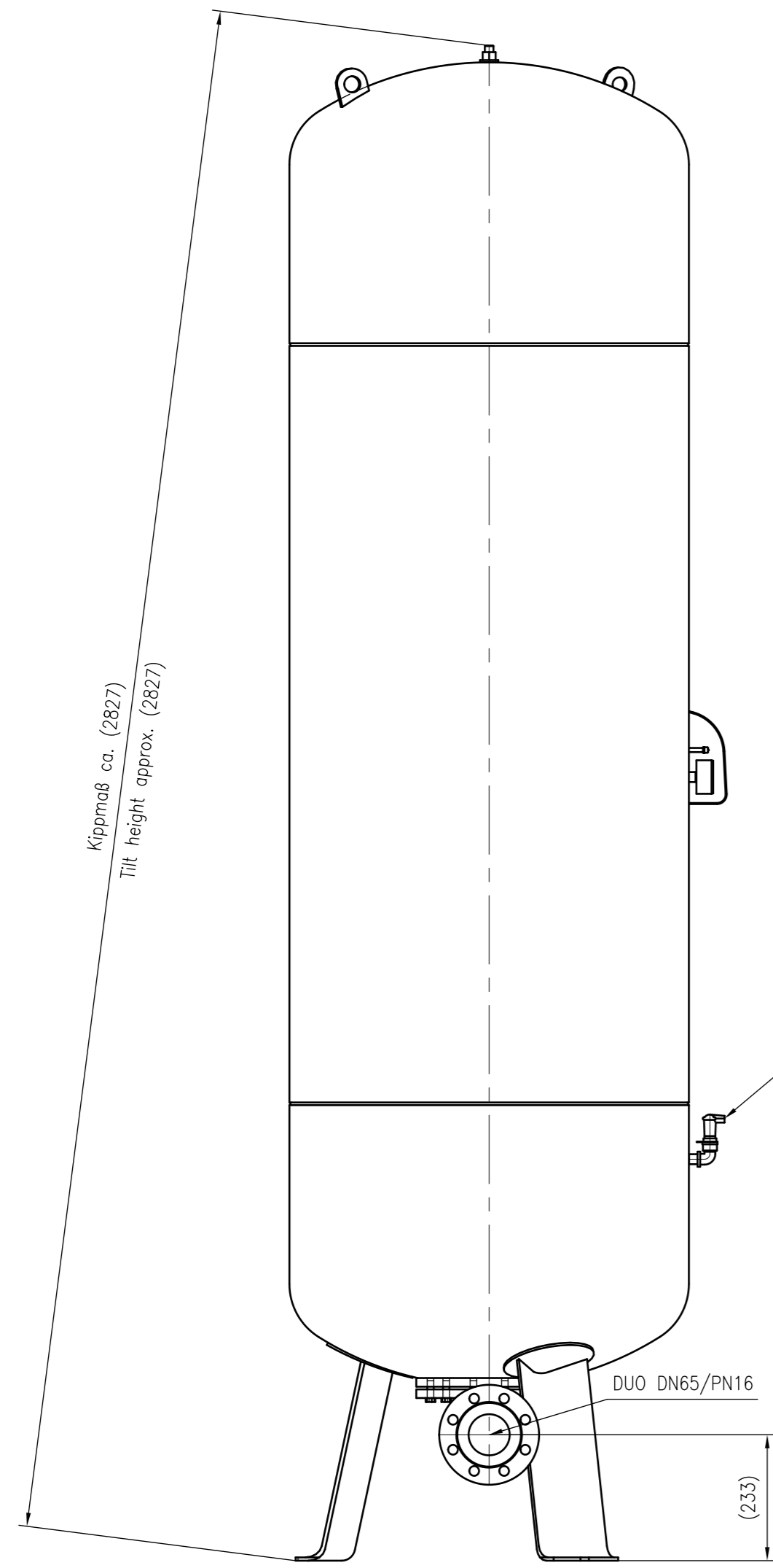
Side view
