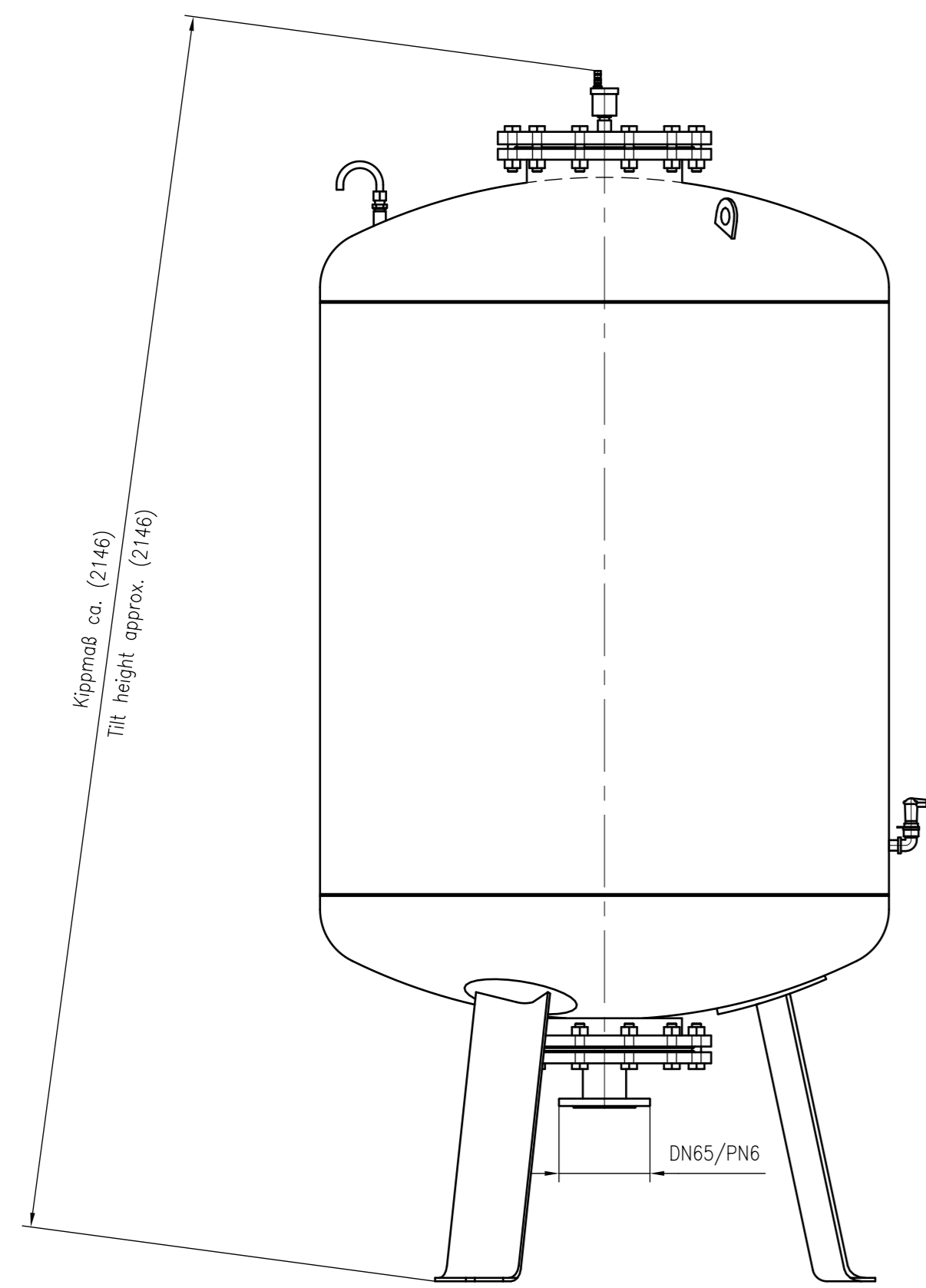
Side view
