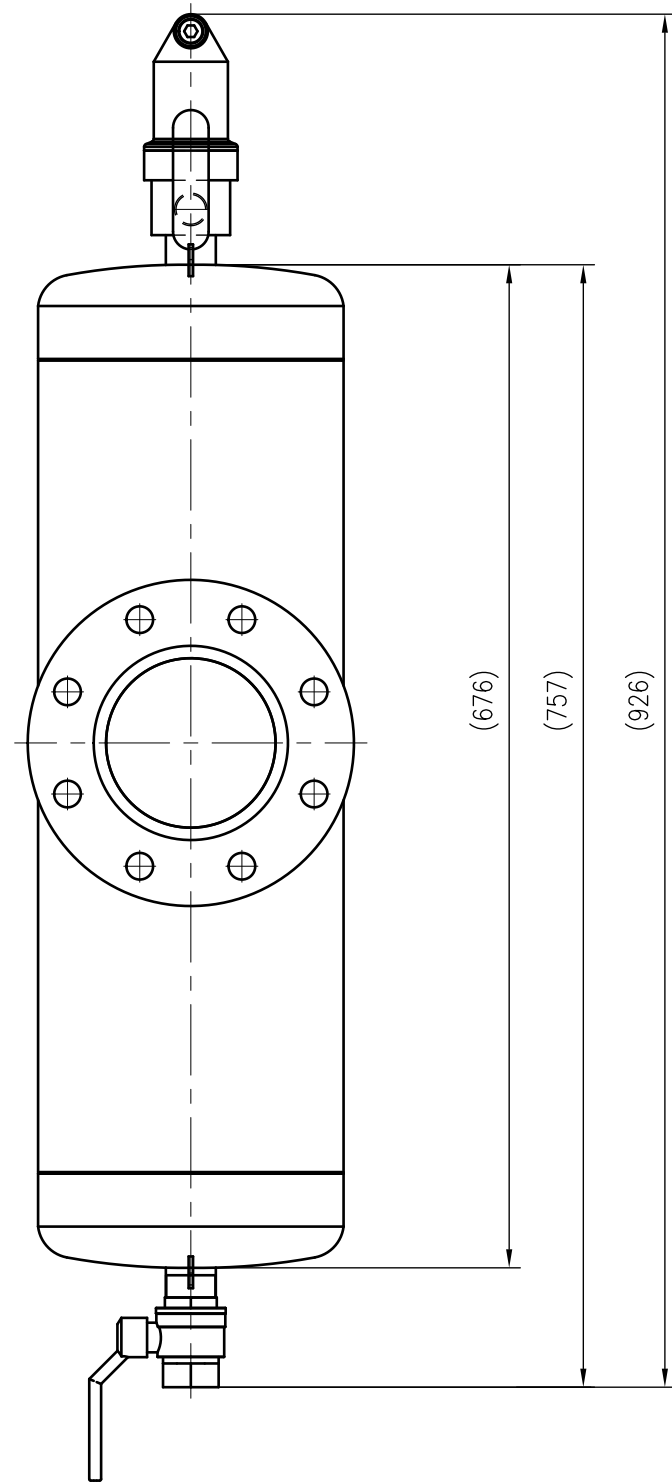
Side view
