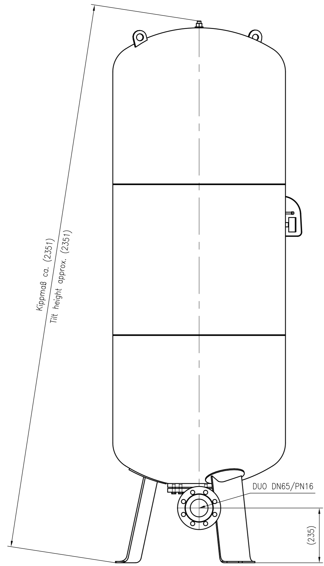
Side view
