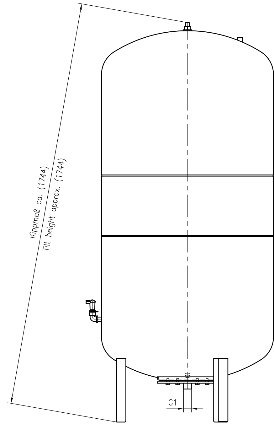
Side view
