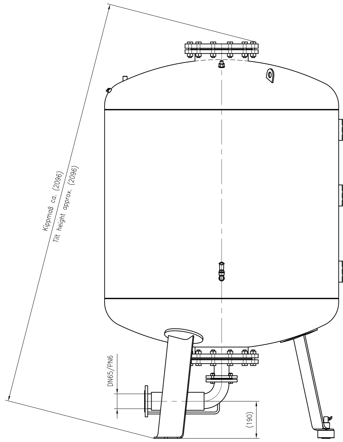
Side view
