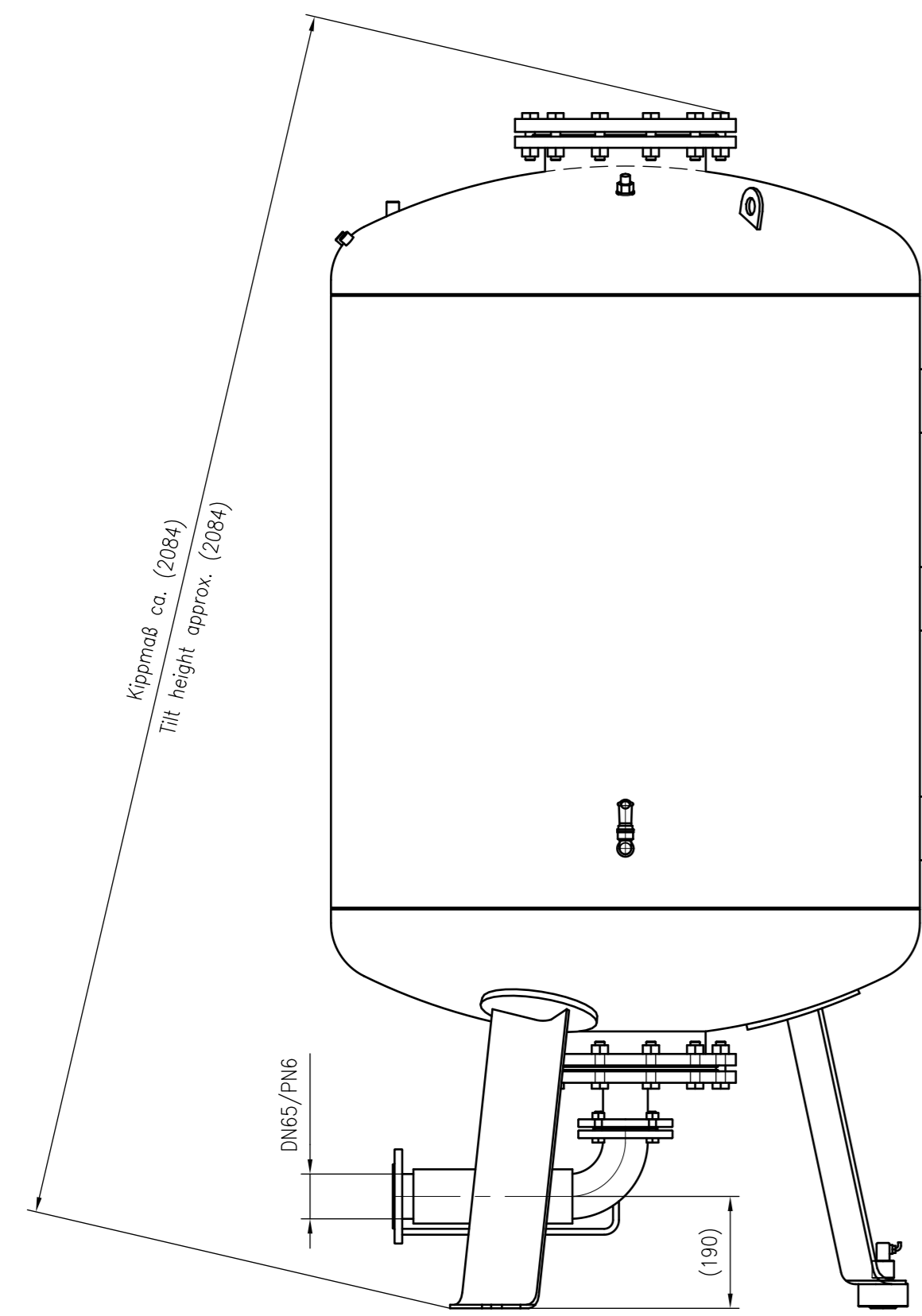
Side view
