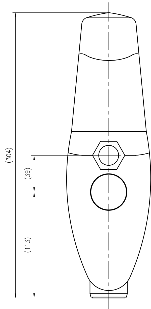
Side view
