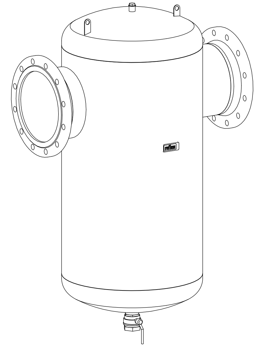
Isometric view
