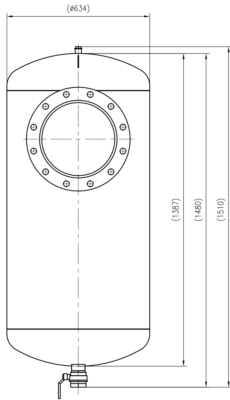
Side view
