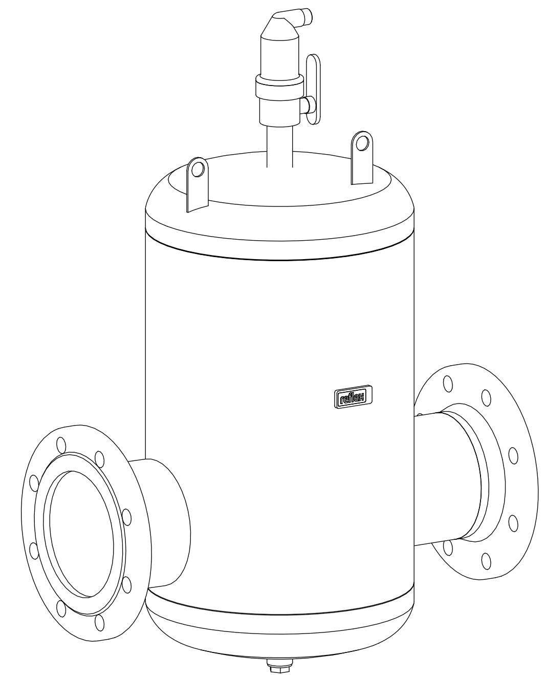
Isometric view
