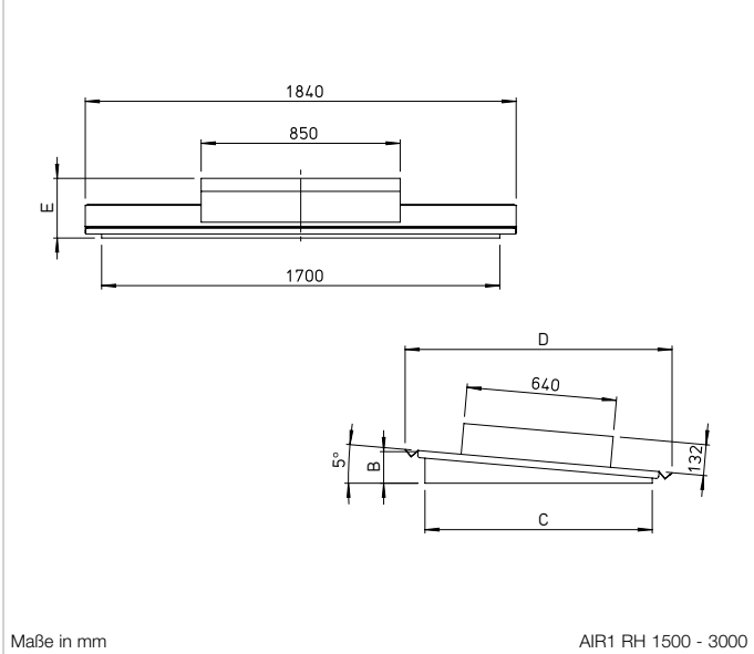
Maße in mm AIR1 RH 1500 - 3000
