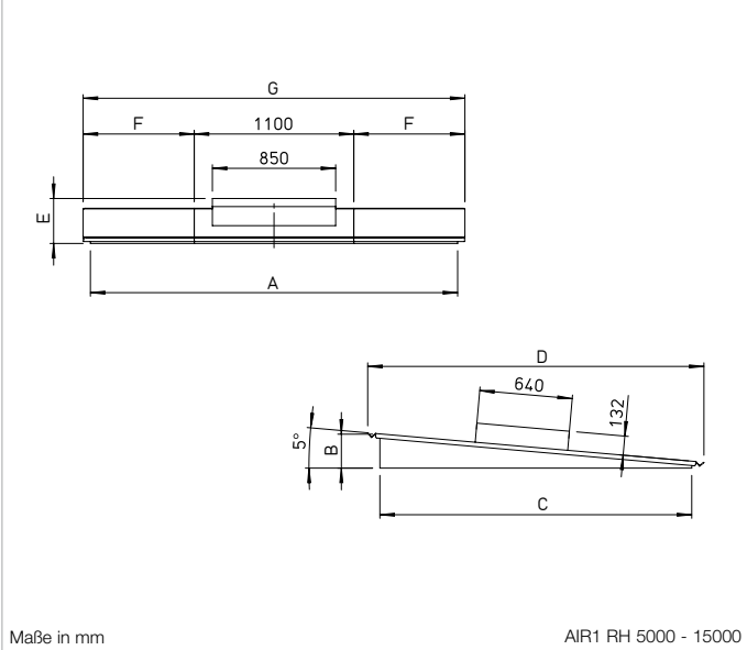
Maße in mm AIR1 RH 5000 - 15000
