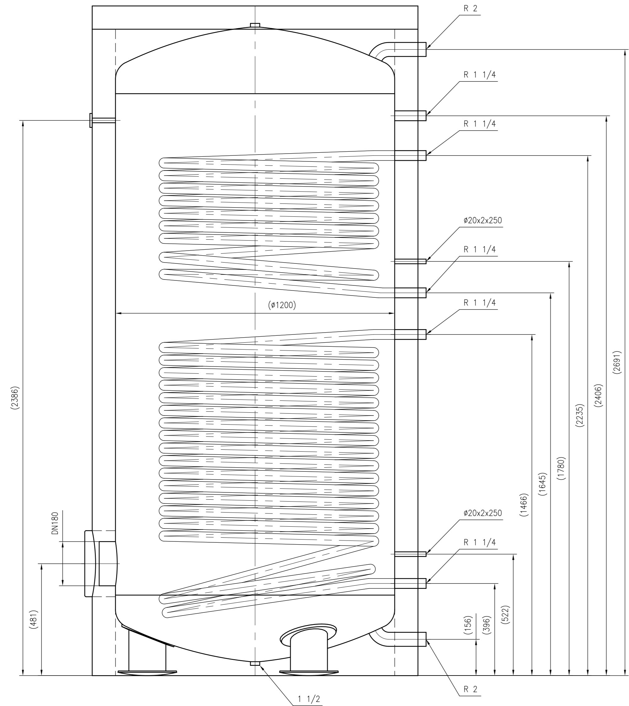
Side view
